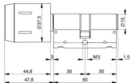
reader knob
