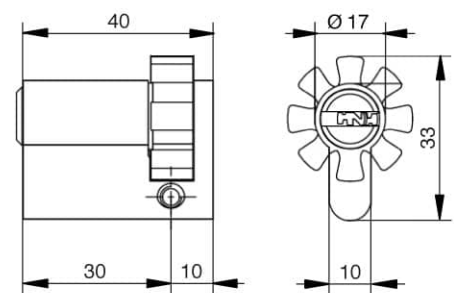
8-way adjustable cam
